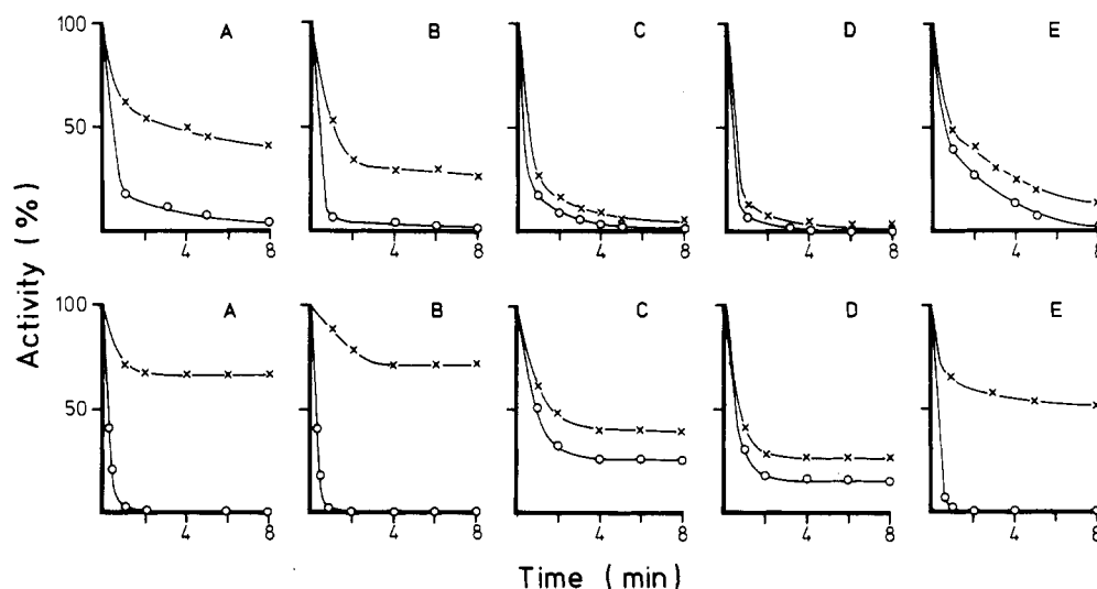
FIGURE 2: (Top row) Influence of diethyl pyrocarbonate treatment on activities of ATP/PP i pyrophosphate exchange (X) and aminoacylation (O) of phenylalanyl-tRNA synthetases from hen liver cytoplasm (A), hen liver mitochondria (B), yeast cytoplasm (C), yeast mitochondria (D), and E. coli (E). A 50-fold excess of diethyl pyrocarbonate, given as molar ratio to total histidine content of the enzyme, was added at 0 °C to absolute protein concentrations of 120–200 µg/mL and incubated for indicated periods of time before assaying. (Bottom row) Influence of phenyl phosphorodichloridate treatment on the activities of ATP/PP i pyrophosphate exchange (X) and aminoacylation (O) of phenylalanyl-tRNA synthetases as given above. Absolute protein concentrations of 120 µg/mL for all enzymes were treated with 1.6 mM reagent at 0 °C and incubated for indicated periods of time before assaying.
