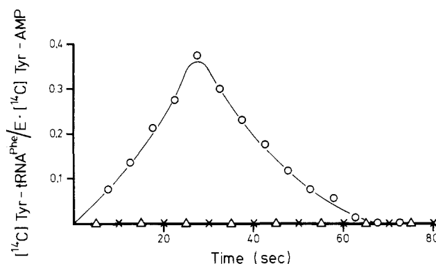
FIGURE 1: Transient formation of 14 C-labeled aminoacyl-tRNA Phe -C-C-A during rejection of phenylalanine analogues by the phenylalanyl-tRNA synthetases of mitochondria from yeast and hen liver at pH 7.65 and 0 °C. Enzyme- 14 C-labeled aminoacyl-AMP (2.8 \mu M) was formed in situ in the presence of inorganic pyrophosphatase. Transfer of [ 14 C]tyrosine to tRNA Phe (7 \mu M) by yeast (O) and hen liver (X) mitochondrial phenylalanyl-tRNA synthetase. Transfer of [ 14 C]tyrosine to tRNA Phe (7 \mu M) by hen liver mitochondrial enzyme with tRNA Phe -C-C-A(3'NH 2 ) ( \Delta ). Aliquots were spotted onto paper filter disks and immediately quenched with trichloroacetic acid.
