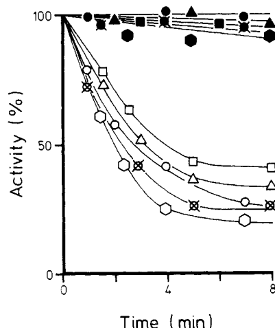
FIGURE 3: Influence of pyridoxal 5'-phosphate on aminoacylation activity of different phenylalanyl-tRNA synthetases. The open symbols correspond to experiments in the absence of tRNA; the full symbols, to the presence of 5 \mu M tRNA Phe . A 5-fold excess of reagent, given as molar ratio to total lysine content of the enzymes, was added at 25 °C to absolute protein concentrations of 100–220 \mu g/mL and incubated for indicated periods of time before assaying. Phenylalanyl-tRNA synthetase from hen liver cytoplasm (crossed open circle, crossed solid circle), hen liver mitochondria (O, ●), yeast cytoplasm (Δ, ▲), yeast mitochondria (□, ■), and E. coli (○, ●).
